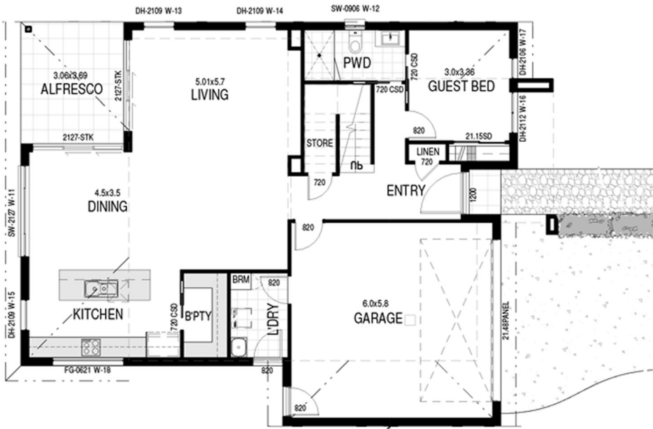
Lower level
